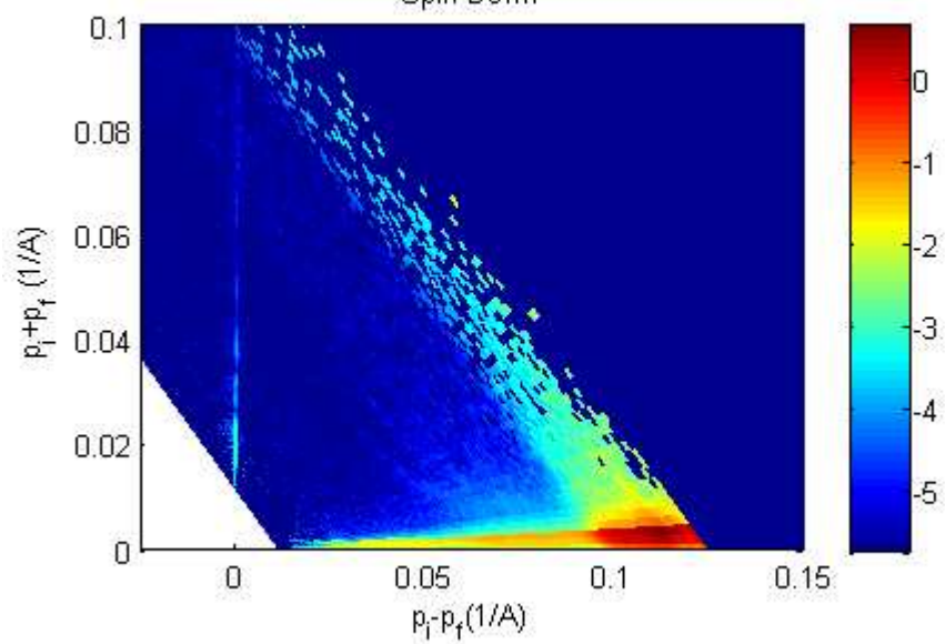
Spin Down
